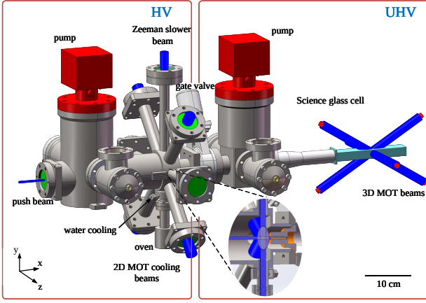
FIG. 1. (Color online) Schematic diagram for the vacuum machine and lasers. The vacuum chamber consists of two parts: the HV where strontium is heated from oven and trapped in a 2D MOT; the UHV for further 3D cooling and operation of tweezer arrays. The size of the entire machine is 500 \times 500 \times 200 mm in xyz axis and its weight is roughly 50 kg.
