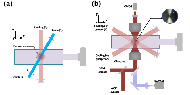
FIG. 3. (Color online) Overview diagram for the tweezer laser setup. (a) Top view of the optical layout. The exciting light, intersects at an angle of approximately 10 degrees with the cooling (MOT) beam (3), and is composed of a pair of counter-propagating probe beams with a frequency offset of approximately 0.5 MHz to avoid the optical interference. The power density of the two probe beams can be meticulously fine-tuned independently, guaranteeing an equilibrium of scattering forces on the atoms during fluorescence imaging. The quantum axis is defined by the polarization of the optical tweezer beam which aligns with the propagating direction of the probe beam, the polarization of probe beams are in the zx plane. (b) The microscope objective possesses a working distance of 15mm, a focal length of 4mm, and a focal depth of 1.5 \mu\text{m} . It is securely affixed to a five-axis electric translation stage (not show). Below the objective lens, the optical tweezer laser and imaging fluorescence are combined with a dichroic mirror. At the top, a camera is used to detect the information of optical tweezers. The inset is the atomic fluorescence excited by a probe beam, propagating from the bottom objective lens to the top. The atomic flux travels in the x axis direction from the 2D MOT.
