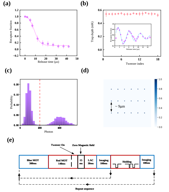
FIG. 5. (Color online) (a). Measured temperature of single atoms trapped in optical tweezers using release and recapture method. Through Monte Carlo simulations, the atoms temperature of the system is approximate 27 \mu K . (b). The trap depth of 18 single atoms in tweezers array. It has a standard deviation of around 1.5% for the tweezer trap depths measured on the atoms transition. The inset shows the measured radial frequency of 103(2) kHz using release and recapture technique. (c). The histogram displays the photon counts of the fluorescence in the region of interest (ROI) of all the single tweezers during the imaging process. Two distinct peaks for vacancy and single atom distribution can be distinctly discerned, which both adhere to a Poisson distribution. The ratio of their integral areas is around 1, indicating a loading efficiency of 0.5. The approximate bin value of the first peak is around 320. The total imaging time is 100ms. (d). Averaged single atoms fluorescence of 50 images. (e). Experimental sequences for the measurement of histogram, lifetime, fluorescence imaging and temperature of the single atoms, and also the trap frequency. The inset sequences in Holding module are corresponding to the measurement of atom temperature and trap frequency. The repump lasers at 679 nm and 707 nm are switched on during the fluorescence imaging in case of the leakage of 1D_2 anti-trapped in 813 nm optical tweezers.
