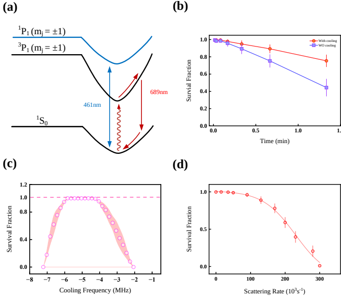
FIG. 4. (Color online) (a). The simplified diagram for broad-line imaging on 1P_1 and narrow-line attractive Sisyphus cooling on the 3P_1 states. The excited state is characterized by a more profound potential depth than that of the ground state. Atoms initially at the trap of ground state, when excited to the excited state, experience a more steep climb than their original state in the ground state. Following spontaneous emission, the disparity between the energy levels leads to a reduction in the atom's average energy [28, 29]. (b). The survival fraction of tweezer array at different trap hold times, with the blue and red curves corresponding to the scenarios with and without Sisyphus cooling, respectively. (c). Depicting the relationship between the survival rate of atoms in the array and the cooling frequency detuning from the AC Stark resonance. (d). The survival fraction of atoms with the rate of scattered 461 nm imaging light with Sisyphus cooling.
