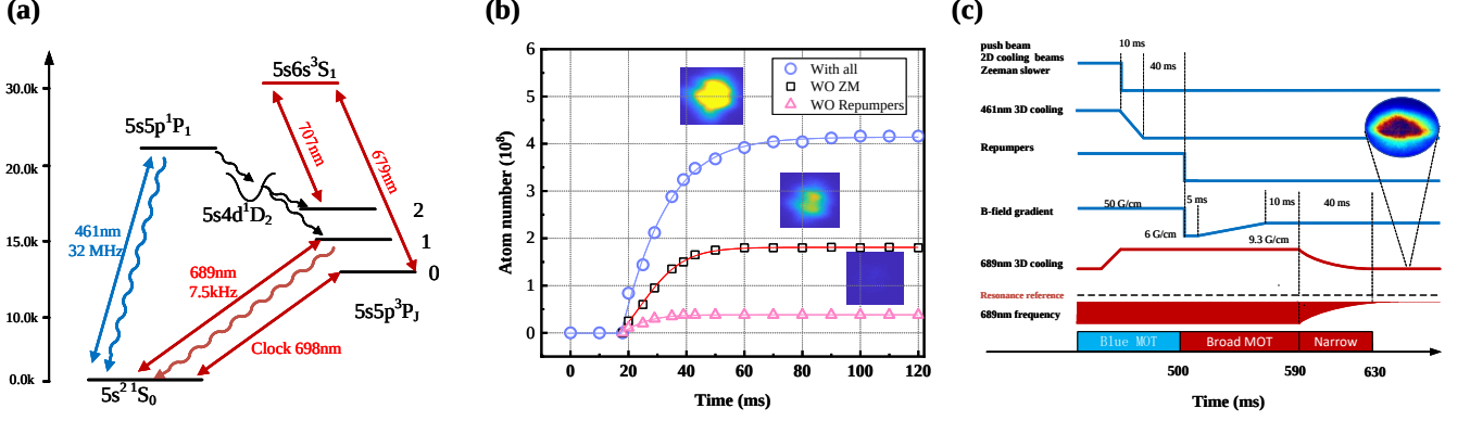
FIG. 2. (Color online) (a) The energy levels for the strontium and the laser system of 461 nm. The blue MOT cooling cycle is composed of a broad cooling transition ^1S_0 \rightarrow ^1P_1 at 461 nm, and two repump transitions ^3P_2 and ^3P_0 \rightarrow ^3S_1 at 707 nm and 679 nm respectively to form a closed cooling transition cycle. (b) The loading rate of blue MOT with/without Zeeman slower (ZM) beams and repumper beams. (c) Time sequence for realizing a narrow red MOT. The inset displays an in-situ image of the compact red MOT.
